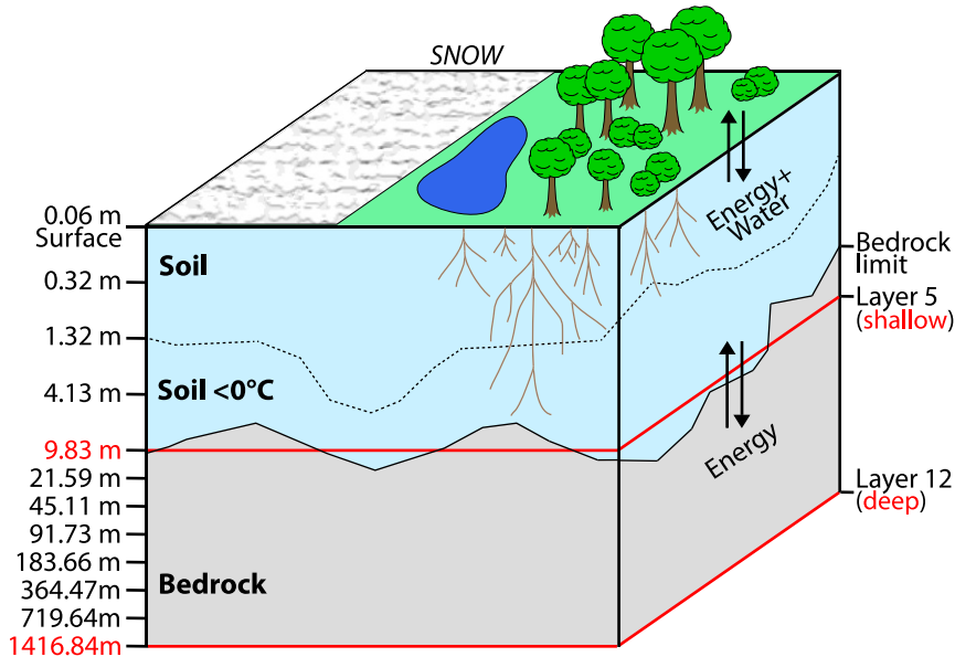
FIG. 1. Vertical structure of the JSBACH LSM version used herein. The scheme corresponds to an example of grid points with frozen soil and partial snow cover, e.g., in northern high latitudes; see also Part II for comparison. The numbers left of the soil column show the depths of the bottom of each layer. Red lines indicate the downward expansion of the BBCP with seven more layers.
